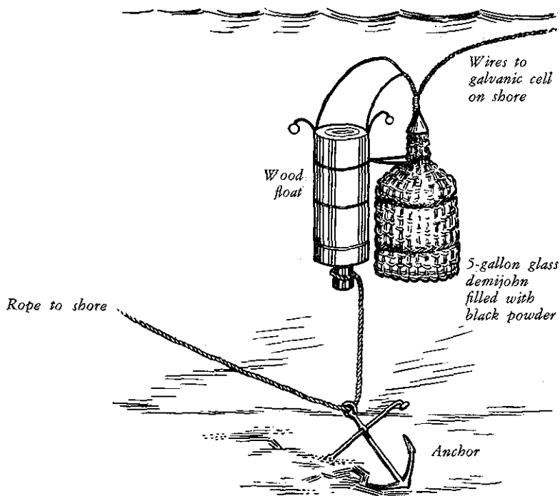
The type of torpedo that sank the U.S.S. Cairo. From a sketch in the Official Records of the Union and Confederate Navies.
