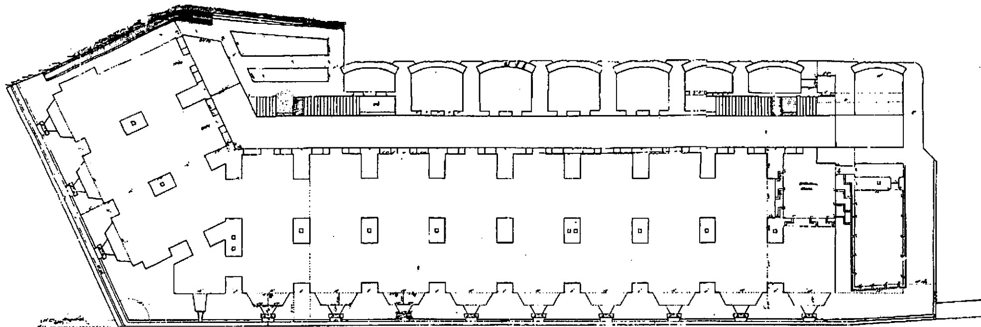
Plan of 2 nd tier - (Quarters)
