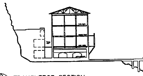
2 TRANSVERSE SECTION 06 SCALE: AS NOTED
