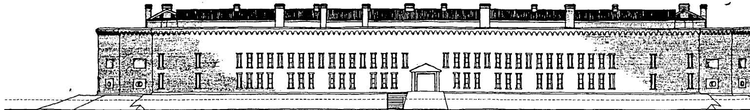
ELEVATION OF GORGE WALL Scale of 1 inch to 16 feet
