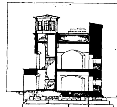
SECTION THROUGH LEFT SHOULDER ANGLE, 1860.
