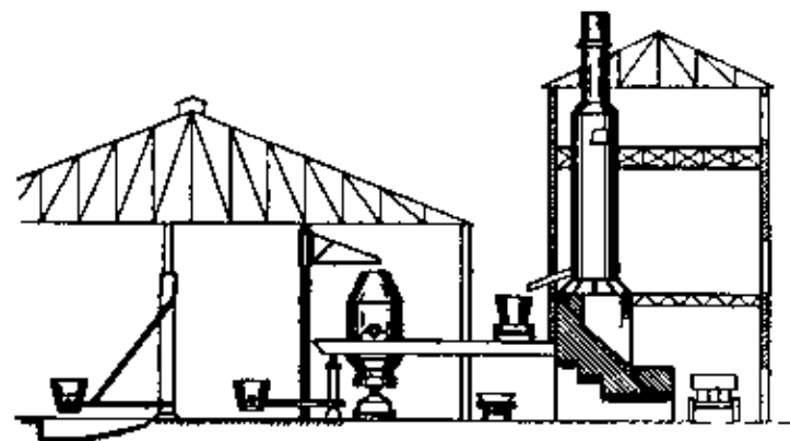
FIG 17—Arrangement of bessemer plant, Cambria Iron Works, 1890.
