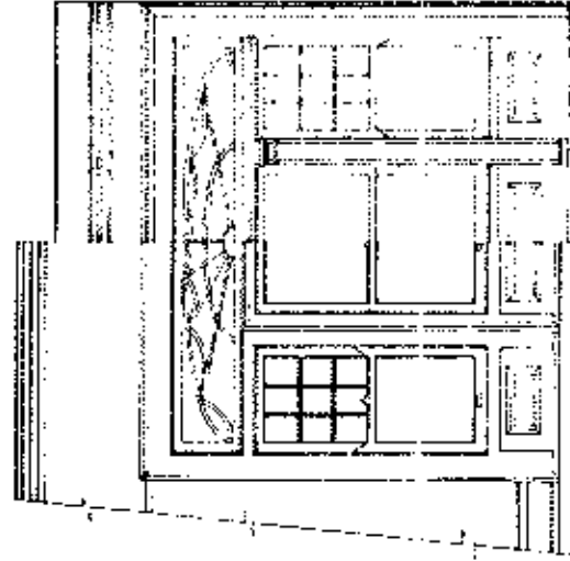
MULTI-PANED WINDOW - INTERIOR/EXTERIOR - SECOND FLOOR, SOUTH ELEVATION
