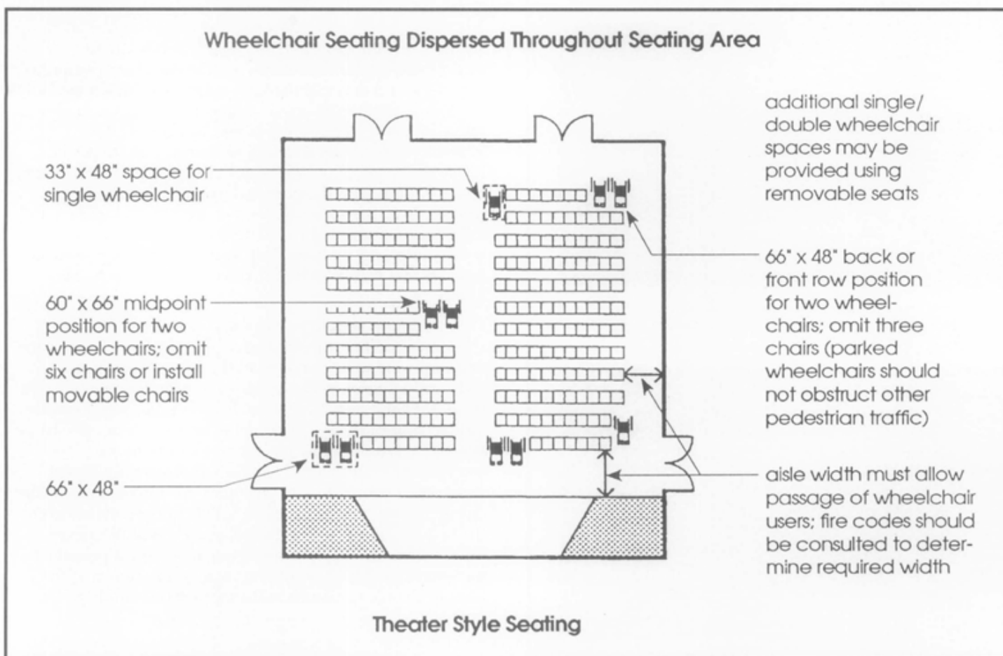
Figure 21. Seating in historic theaters and auditoriums can be changed to accommodate wheelchair users. Accessible seating areas should be connected to an accessible route from the building entrance. Source: UFAS Retrofit Manual.
